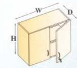
Over Head Storage W=600,750,900,1050,1200 D=300,350,380,400,450 H=450,600,750,800,900
