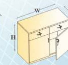
Side Cabinet W=600,750,900 D=400,450 H=750,900
