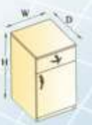
Free Standing Pedestal (1D/1S) W=400,450 D=400,450,500,550,600 H=700,725,750
