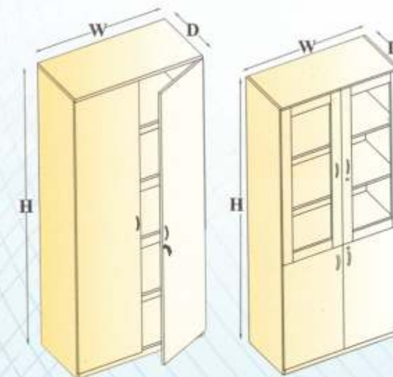
High Swing Door W=600,750,900 D=400,450,500,550,600 H=1650,1800,2100
