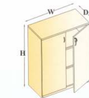
Medium Swing Door (2S) W=600,750,900 D=400,450,500,550,600 H=1175,1200,1350,1500
